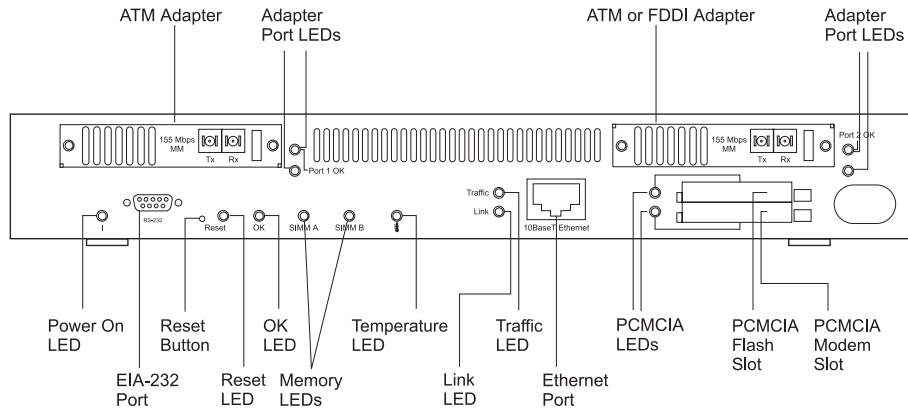
Figure 1-1. Front Panel of the IBM 8210-003
