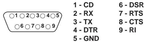
Figure 3-1. EIA-232, Service-Port, Pin Assignments
